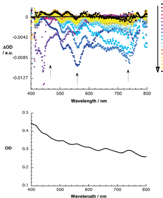
Figure 3. Differential absorption spectra (top; visible) obtained upon femtosecond flash photolysis (387 nm) of \text{SWNT-PSS}^{n-} in nitrogen-saturated aqueous solutions with several time delays between 0 and 5 ps at room temperature (arrows indicate the evolution of differential changes) and absorption spectrum (bottom) of \text{SWNT-PSS}^{n-} .
