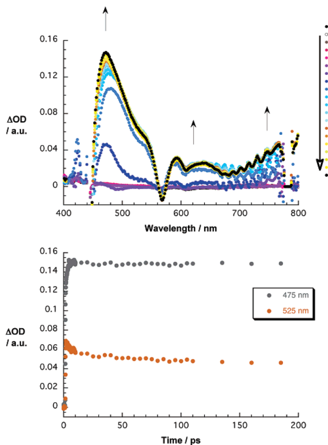
Figure 2. Differential absorption spectra (top; visible) obtained upon femtosecond flash photolysis (387 nm) of \text{ZnP}^{8-} in nitrogen-saturated aqueous solutions with several time delays between 0 and 5 ps at room temperature (arrows indicate the evolution of differential changes) and time-absorption profiles (bottom) of the porphyrin shown above at 475 and 525 nm, monitoring the decay of the porphyrin singlet excited state.
